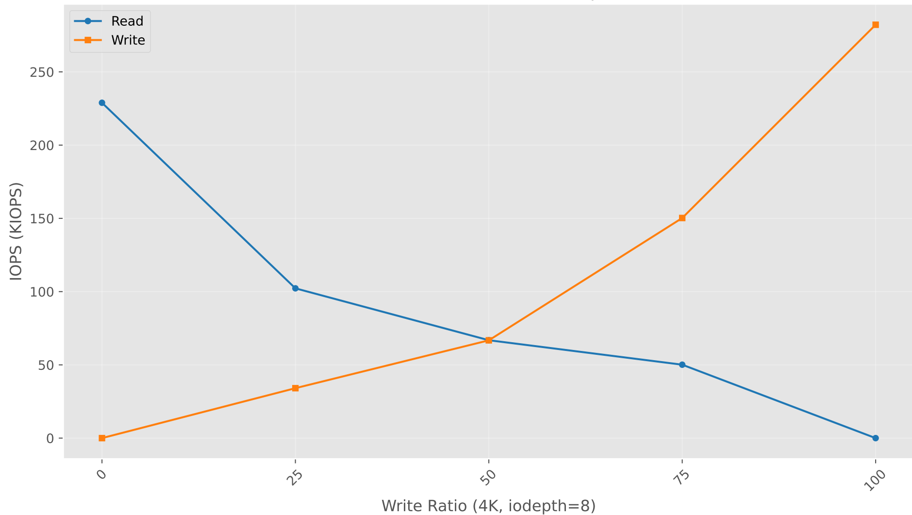
IOPS vs Write Ratio (4K, iodepth=8)
